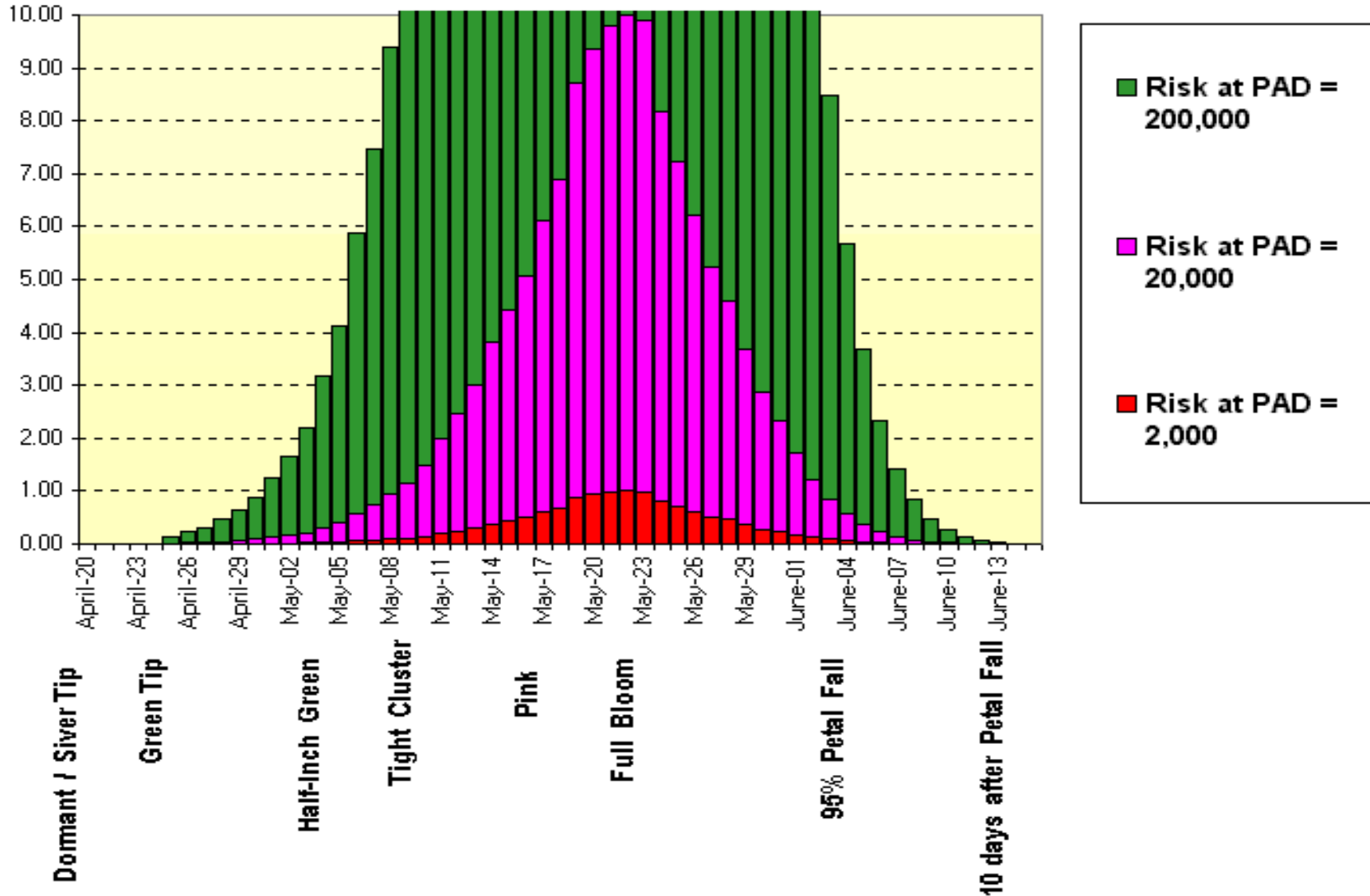
Average Primary Scab Risk by Growth Stage
